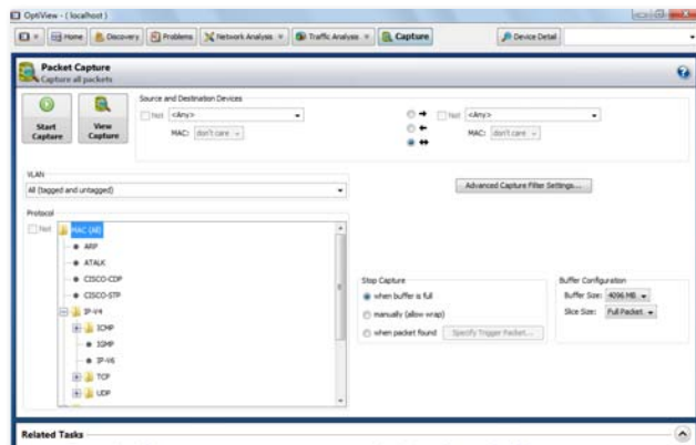
Packet capture
