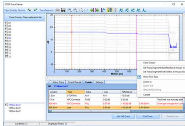
Setting span event parameters using LinkWare PC
