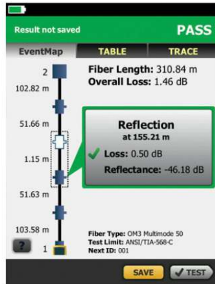
Graphical EventMap view – PASS
