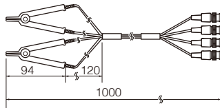
FOUR-TERMINAL PROBE 9140-10
