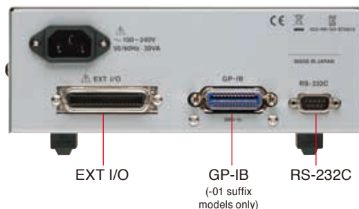
3561-01 Rear Panel
