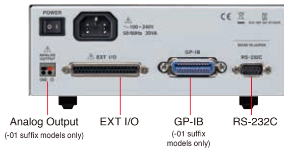
3561-01 Rear Panel
