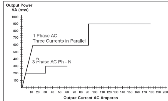
Current Amplifier Output Power Curve
