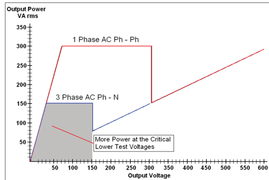
"PowerV" Voltage Amplifier Output Power Curves
